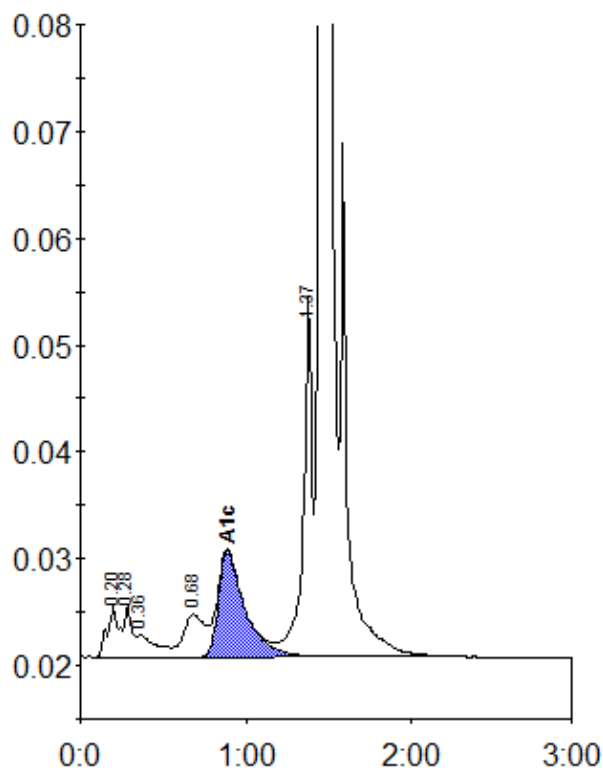
Peak table - ID: 10404321
